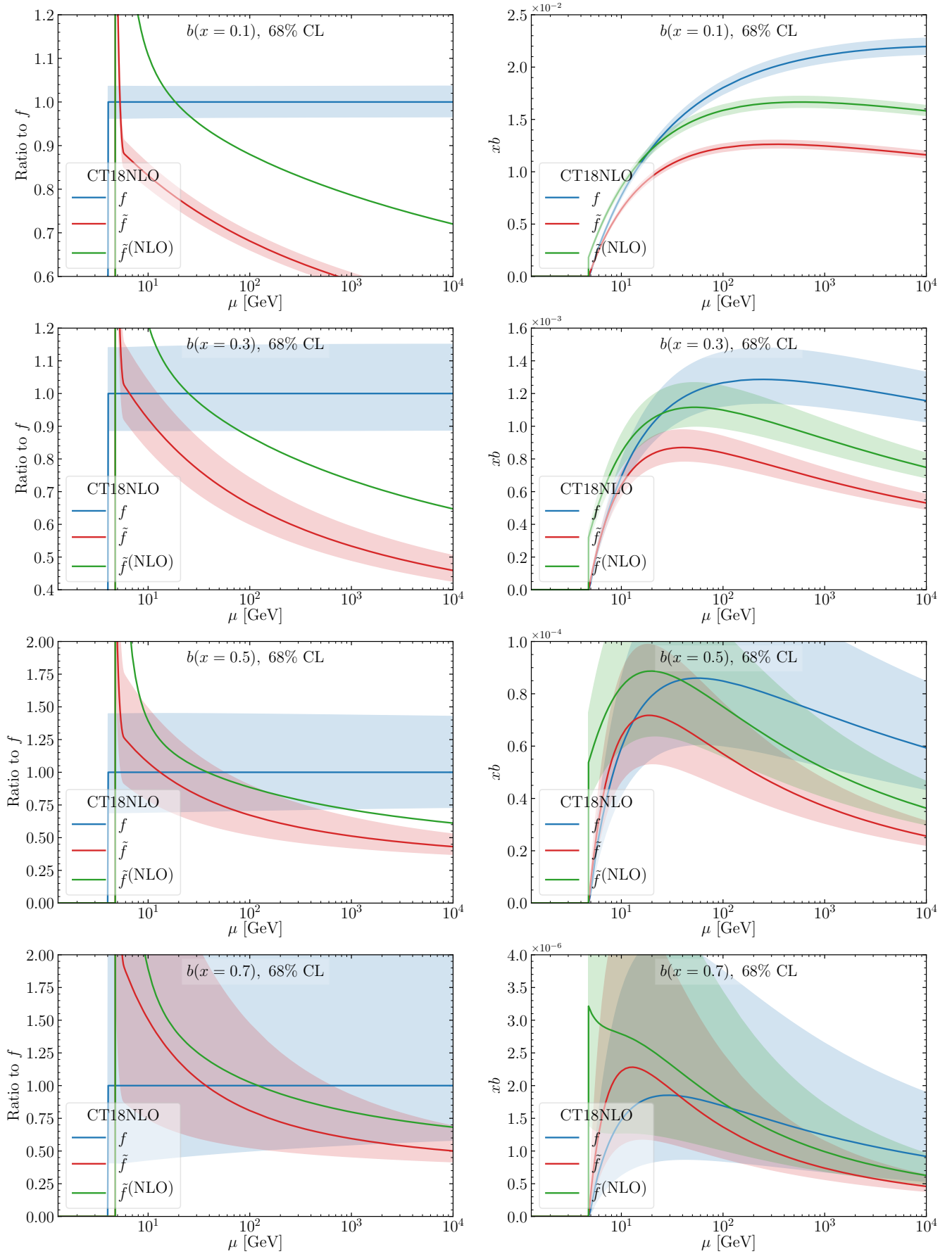
FIG. 1: CT18NLO_Bsub_xs: CT18NLO_CT18NLO_Bsub_CT18NLO_Bsub_nlo_x0p7_05_xbqk_liny
