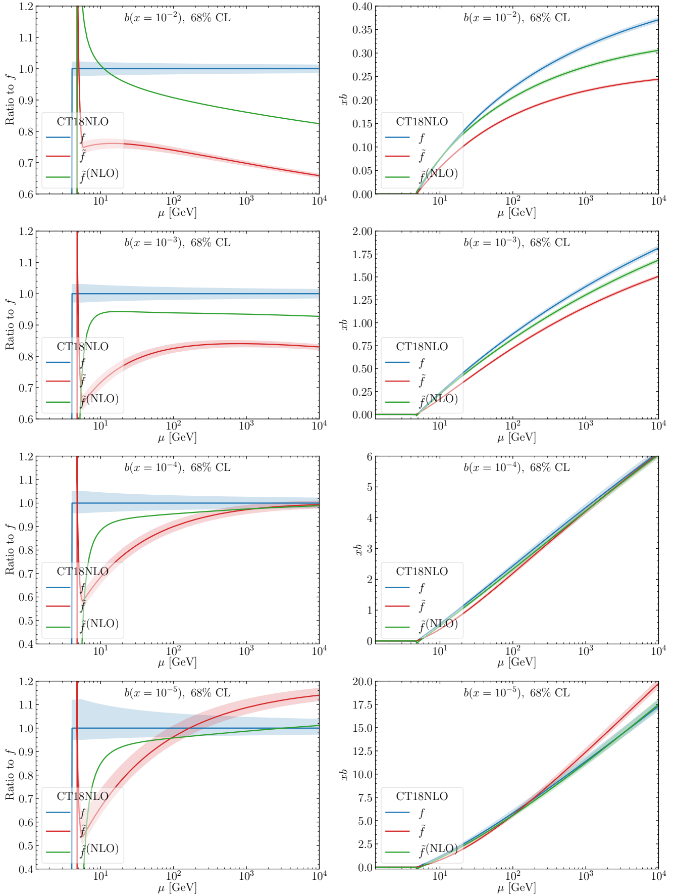
FIG. 2: CT18NLO_Bsub_xs: CT18NLO_CT18NLO_Bsub_CT18NLO_Bsub_nlo_x1e-5_05_xbqk.liny
